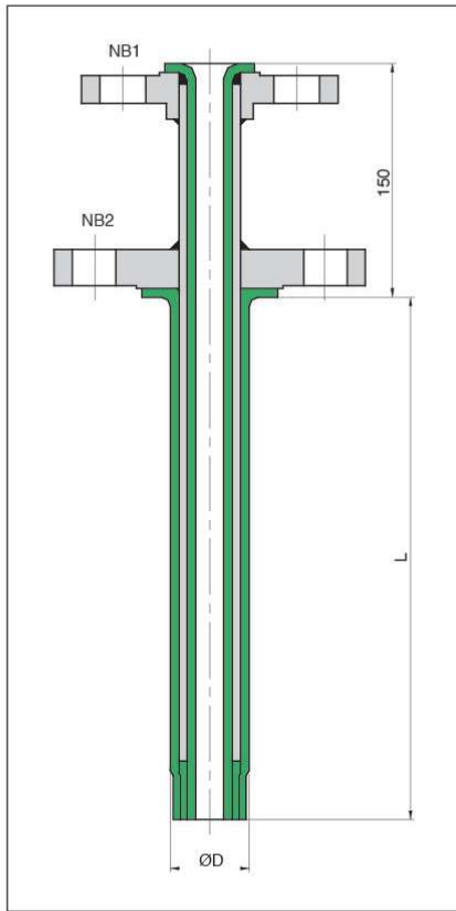
Welded Flange Type
