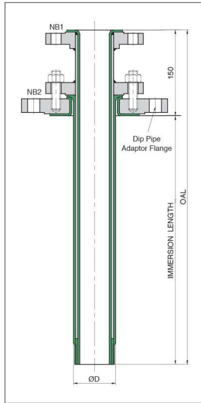
Reducing Flange Type
