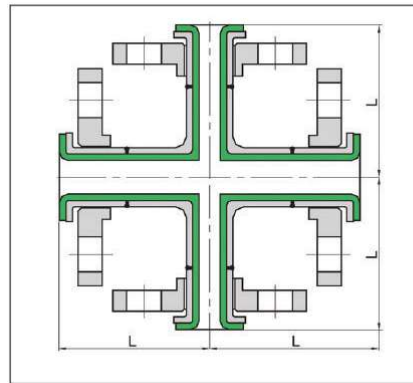
Steel Equal Cross, LF
