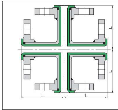
Equal Cross, FF
