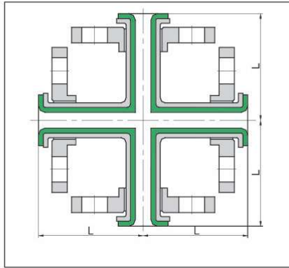
Equal Cross, LF
