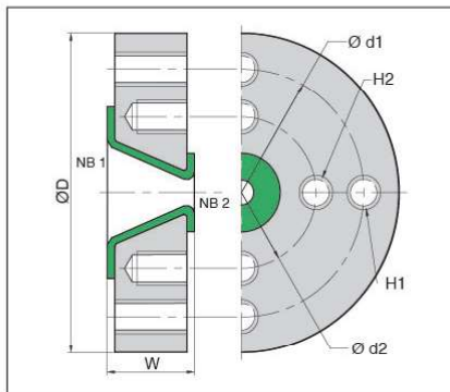
Reducing Flange Type 3
