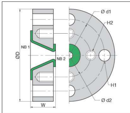
Reducing Flange Type 1
