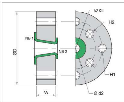
Reducing Flange Type 2
