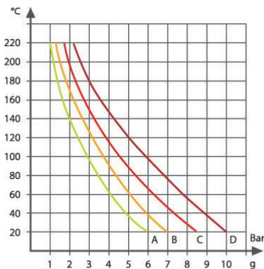
Pressure Resistance (3 Convolutions) Type APBS
