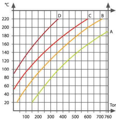
Vacuum Resistance Type APBS
