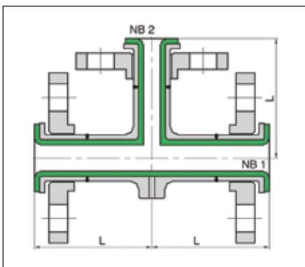
Steel Red Tee, LF
