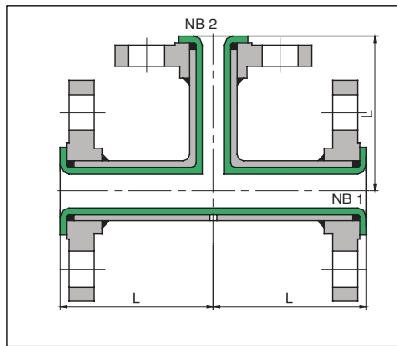
Red Tee, FF
