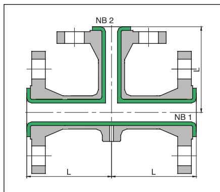
Cast Steel Red Tee, FF
