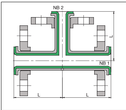
Stub-End Red Tee, LF
