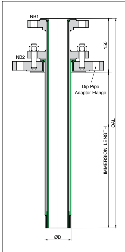
Reducing Flange Type
