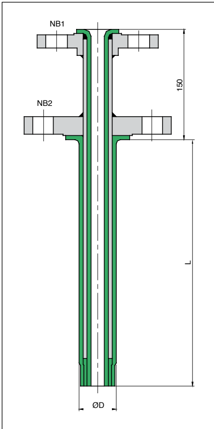
Welded Flange Typet
